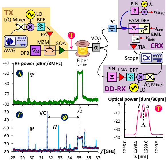
Fig. 2: Setup and transmitted RF / optical spectra.
